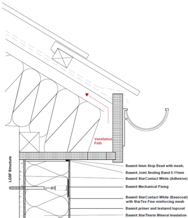
Diagram 6 - Typical overhanging eaves detail
