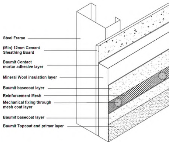
Diagram 2 - Typical build up detail
