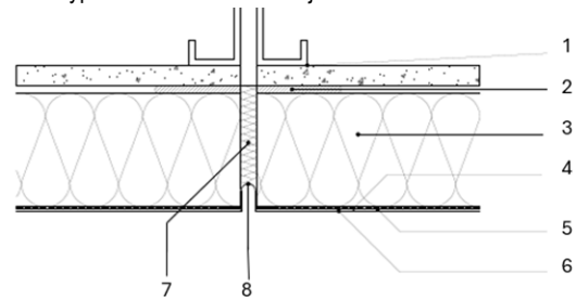
Diagram 3 - Typical vertical movement joint detail
