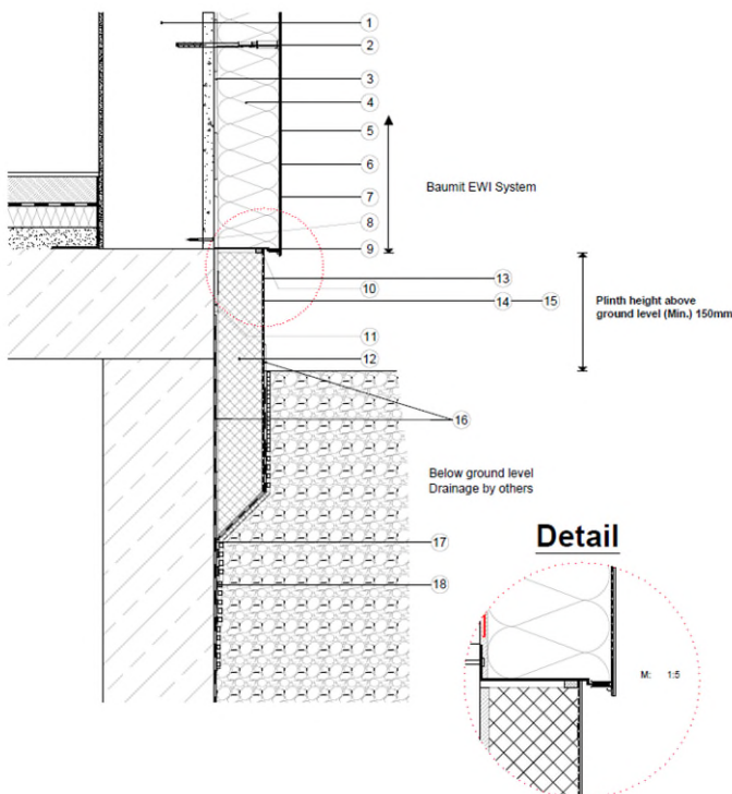
Diagram 3 - Typical standard base detail
