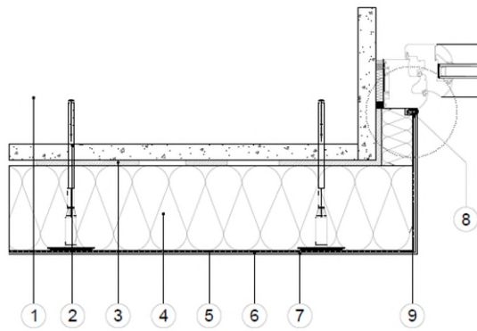
Diagram 4 - Typical window reveal detail
