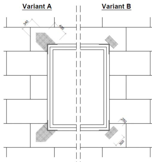
Diagram 7 - Typical opening stress patch detail
