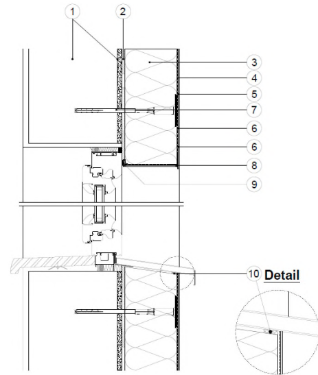
Diagram 5 - Typical window head and cill detail
