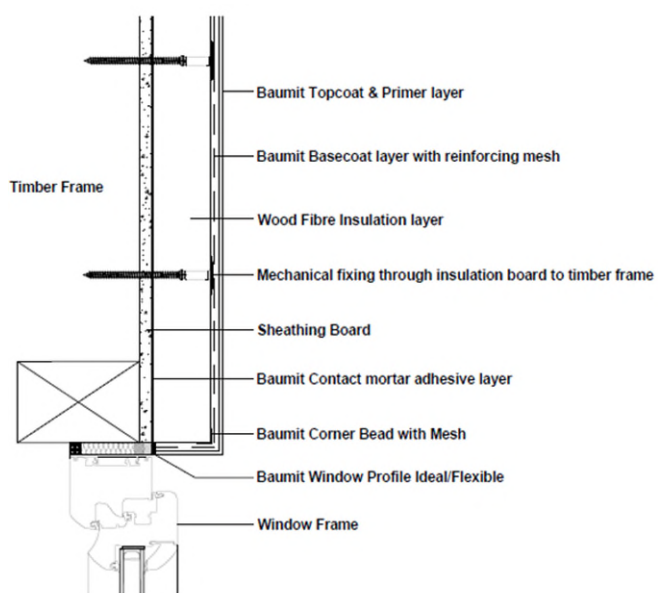
Diagram 6 - Typical window reveal detail
