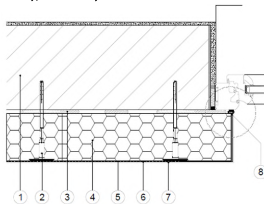
Diagram 6 - Typical window jamb detail
