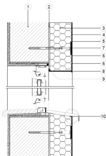
Diagram 5 - Typical window head detail
