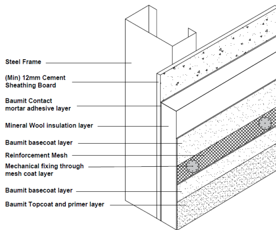
Diagram 2 - Typical build up detail
