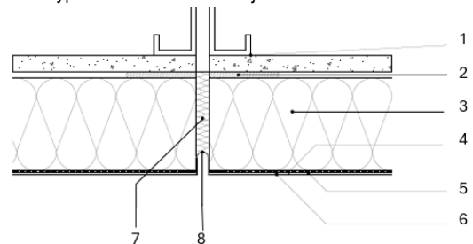
Diagram 3 - Typical vertical movement joint detail
